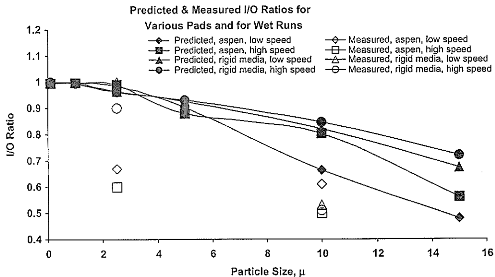
Fig. 11. Comparison of predicted and measured I/O ratios for wet runs.
