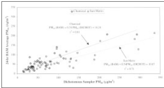
Figure 3. Comparison of PM_{10} concentrations acquired by the dichotomous monitor and BAM at Chamizal and Sun Metro for the period of December 2, 1999, to March 7, 2000. All concentrations were reported under STP conditions.
